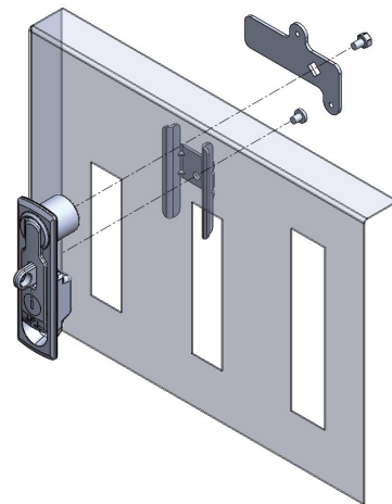
Installation Method
