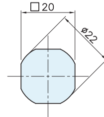
PANEL DRILLING DIMENSIONS.
