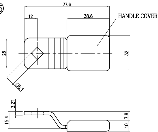
KA-619-1K,2K (SCP)
