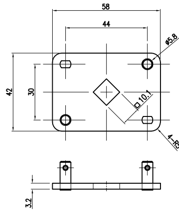
KA-615 (SCP)
