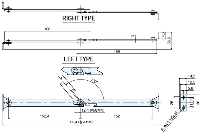
SCALE 1 : 1 KD-1102-1(정면)
